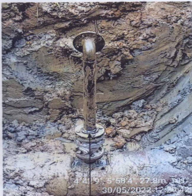
SPILL POINT ( After excavation: Installed 3" ball valve At 12 O'clock position on the pipeline )
